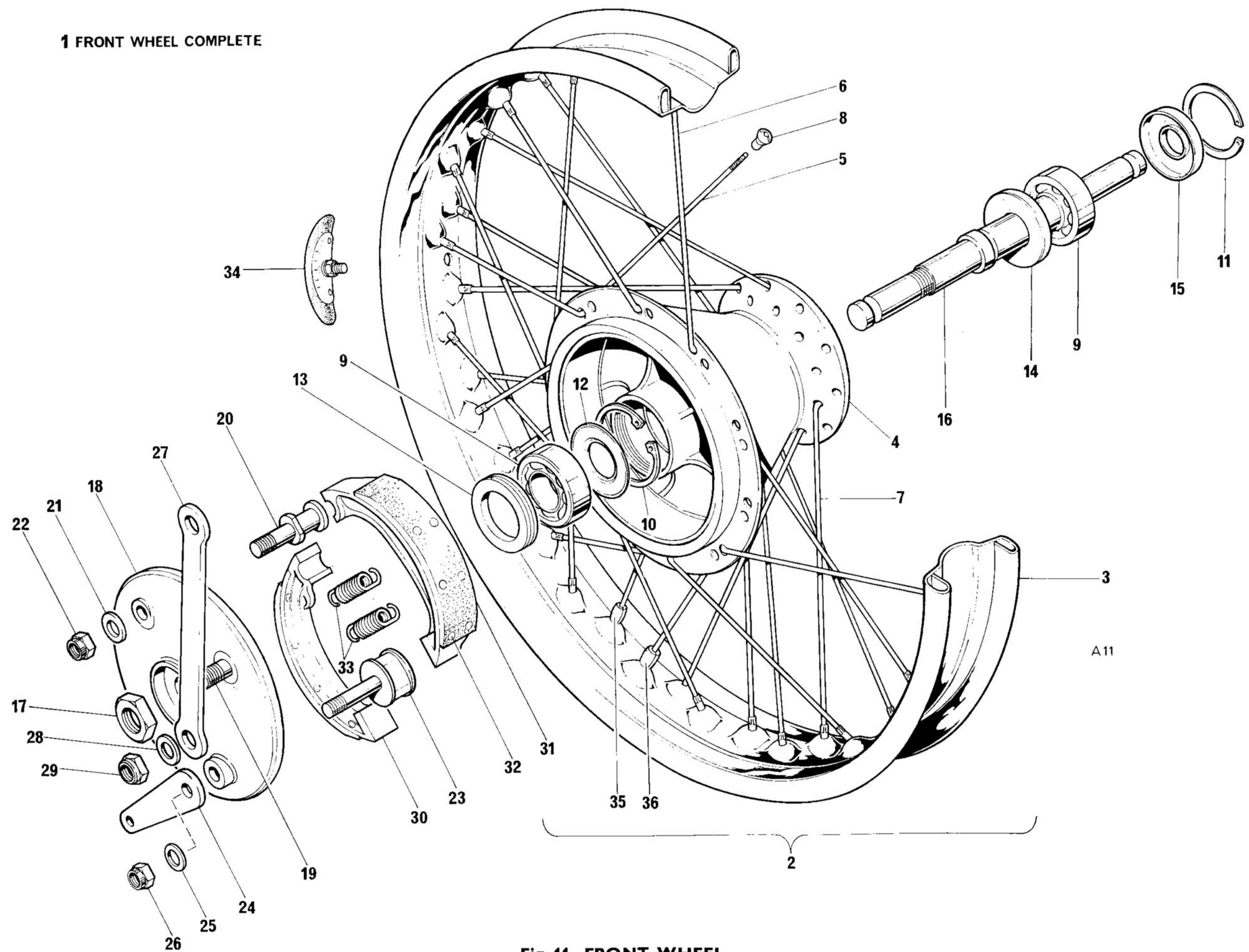
Fig. 11. FRONT WHEEL
