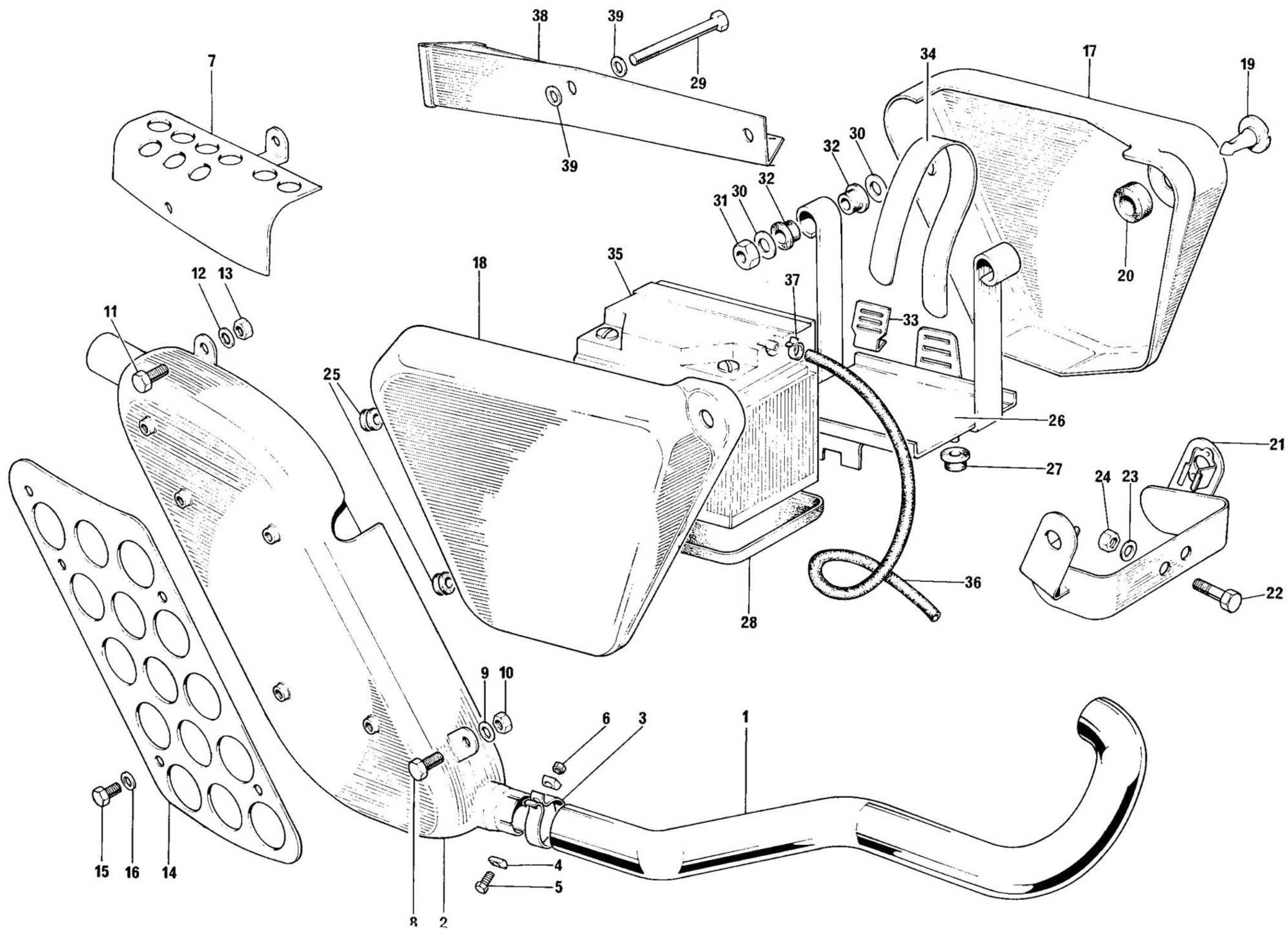
Fig. 7. EXHAUST SYSTEM, SIDE COVERS AND BATTERY
