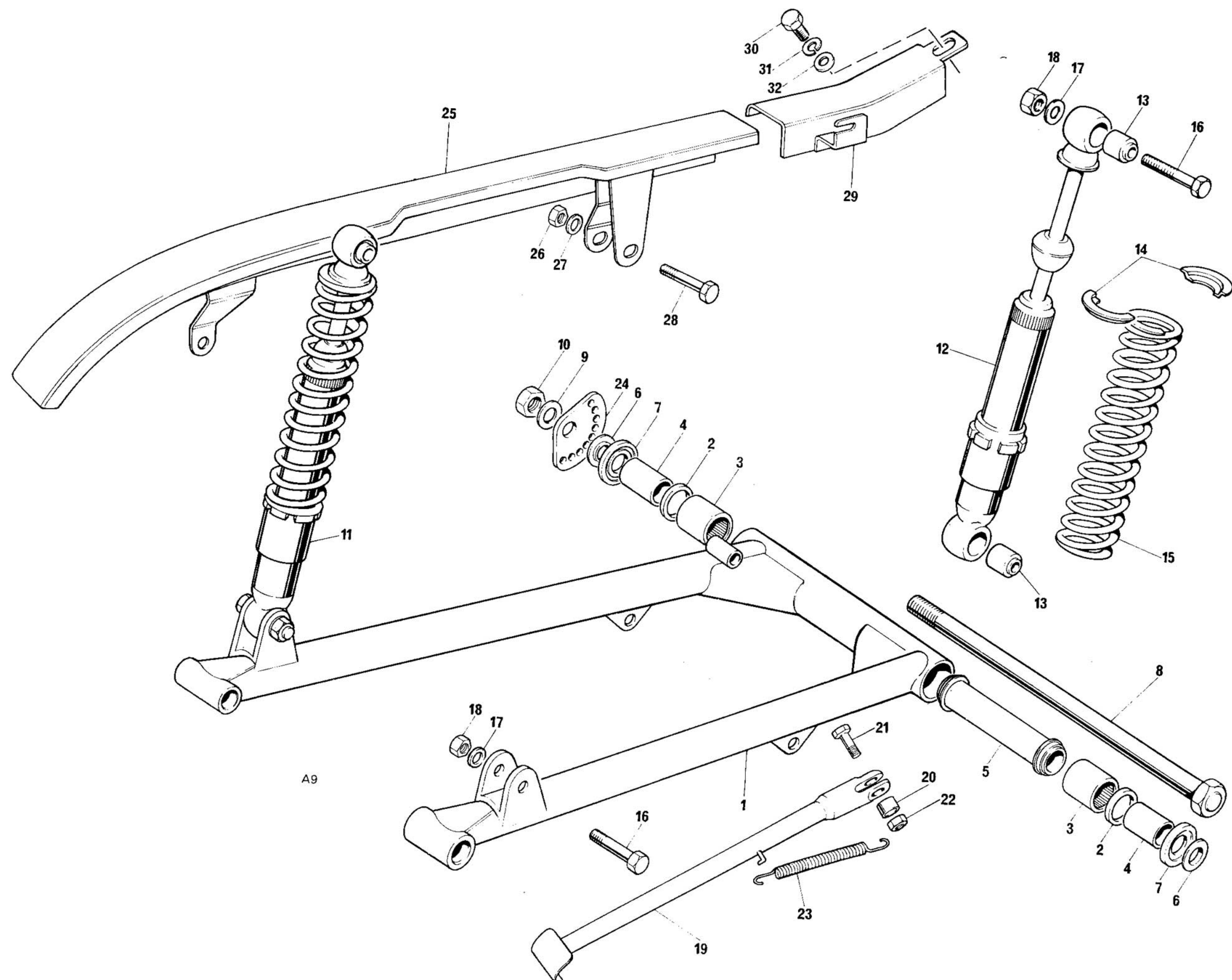
Fig. 9. SWINGING ARM AND SUSPENSION UNITS
