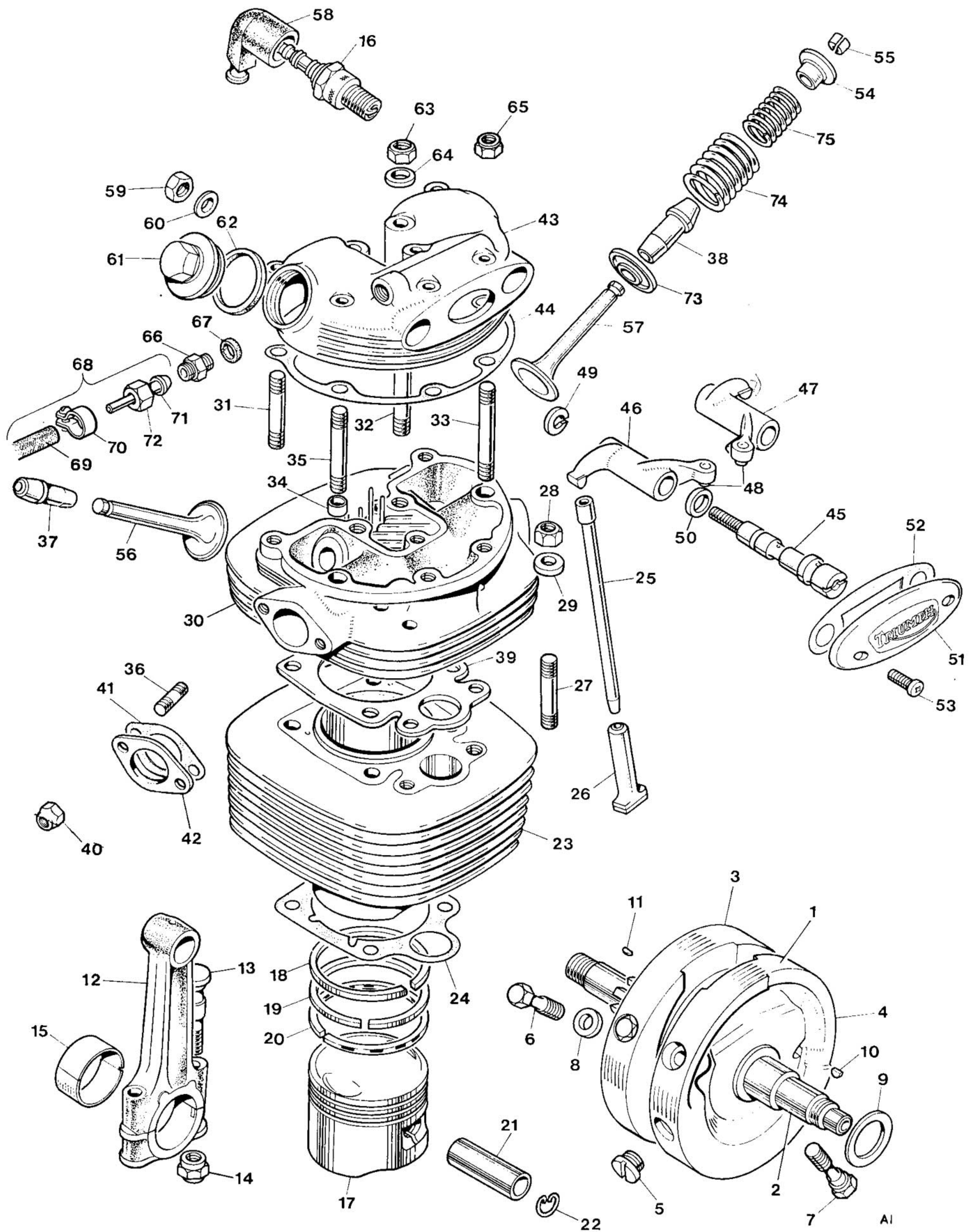
Fig. 1. CYLINDER HEAD, BARREL AND CRANKSHAFT
