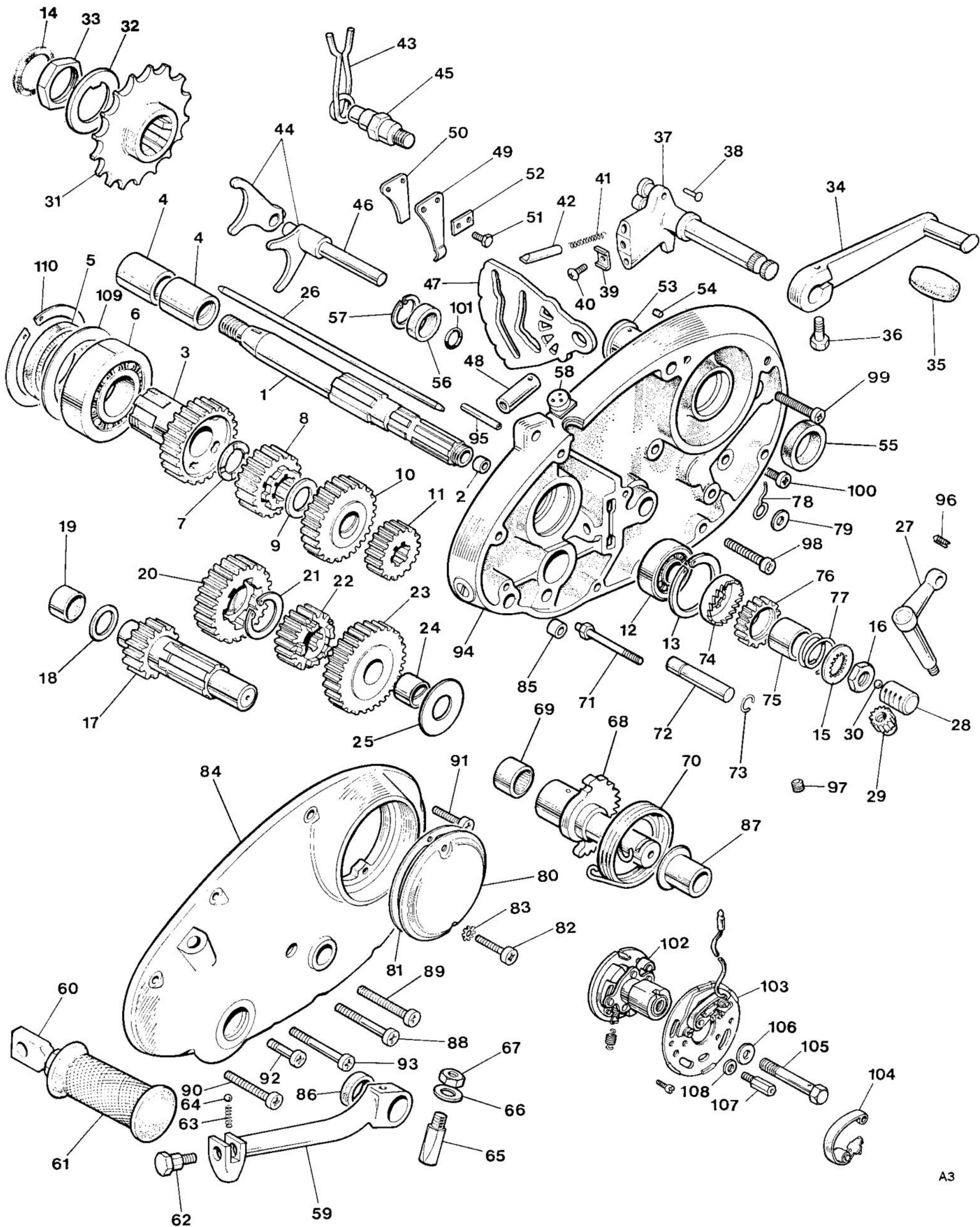
Fig. 4. GEAR CLUSTERS AND TIMING COVERS
