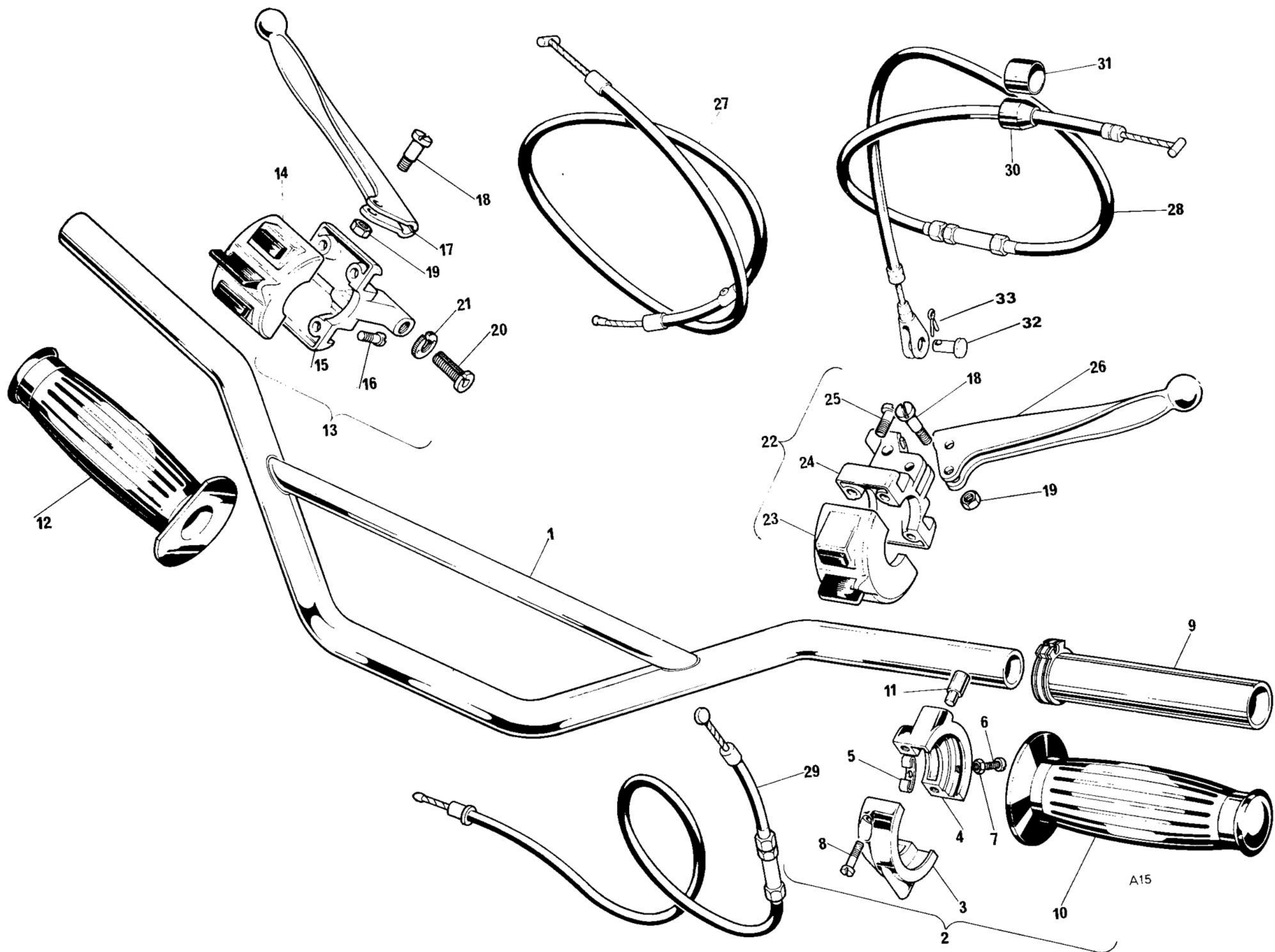
Fig. 15. HANDLEBARS, CONTROL LEVERS AND CABLES
