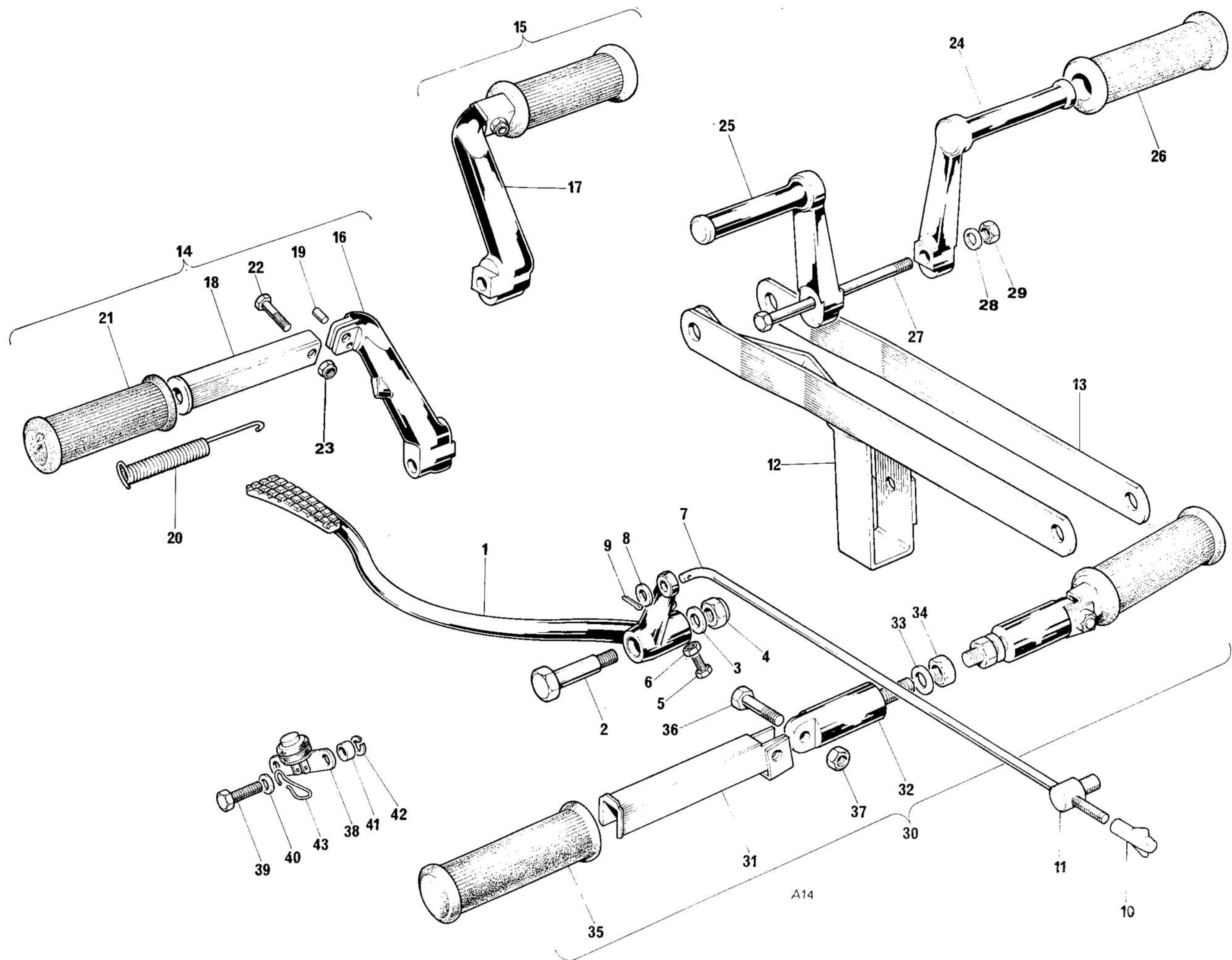
Fig. 14. BRAKE PEDAL AND FOOTRESTS
