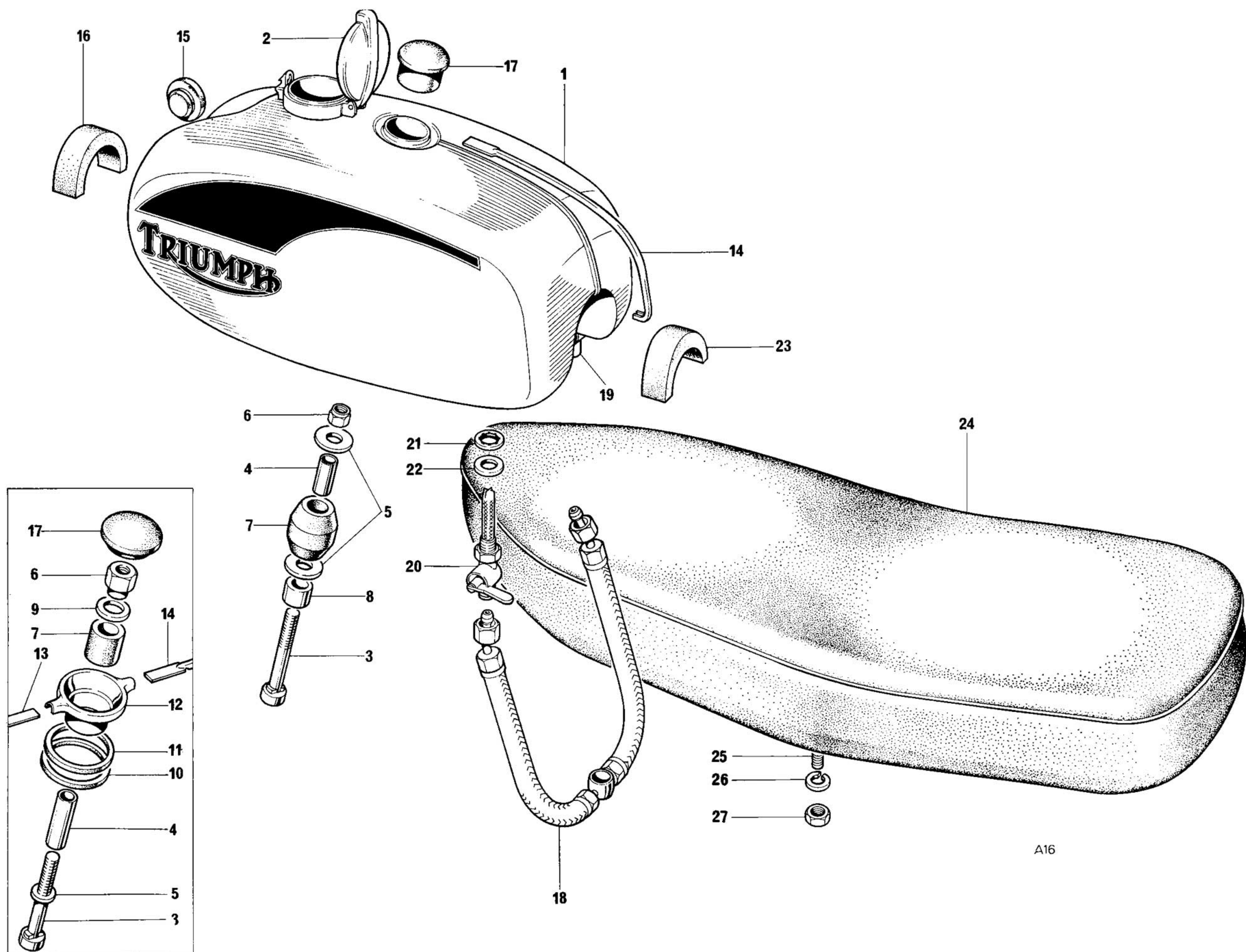
Fig. 16. GAS TANKS AND TWINSEAT
