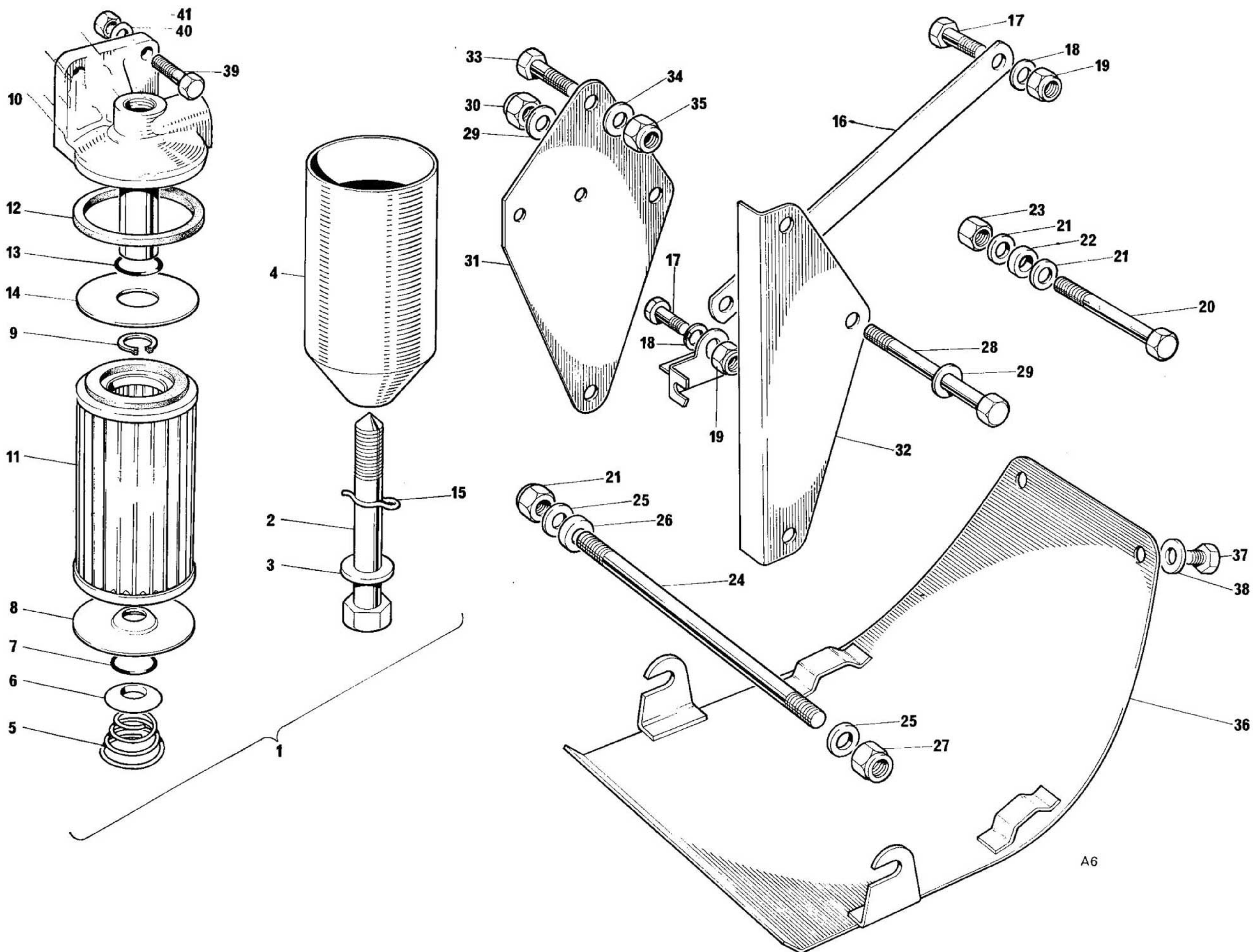
Fig. 6. OIL FILTER, MOTOR FIXINGS
