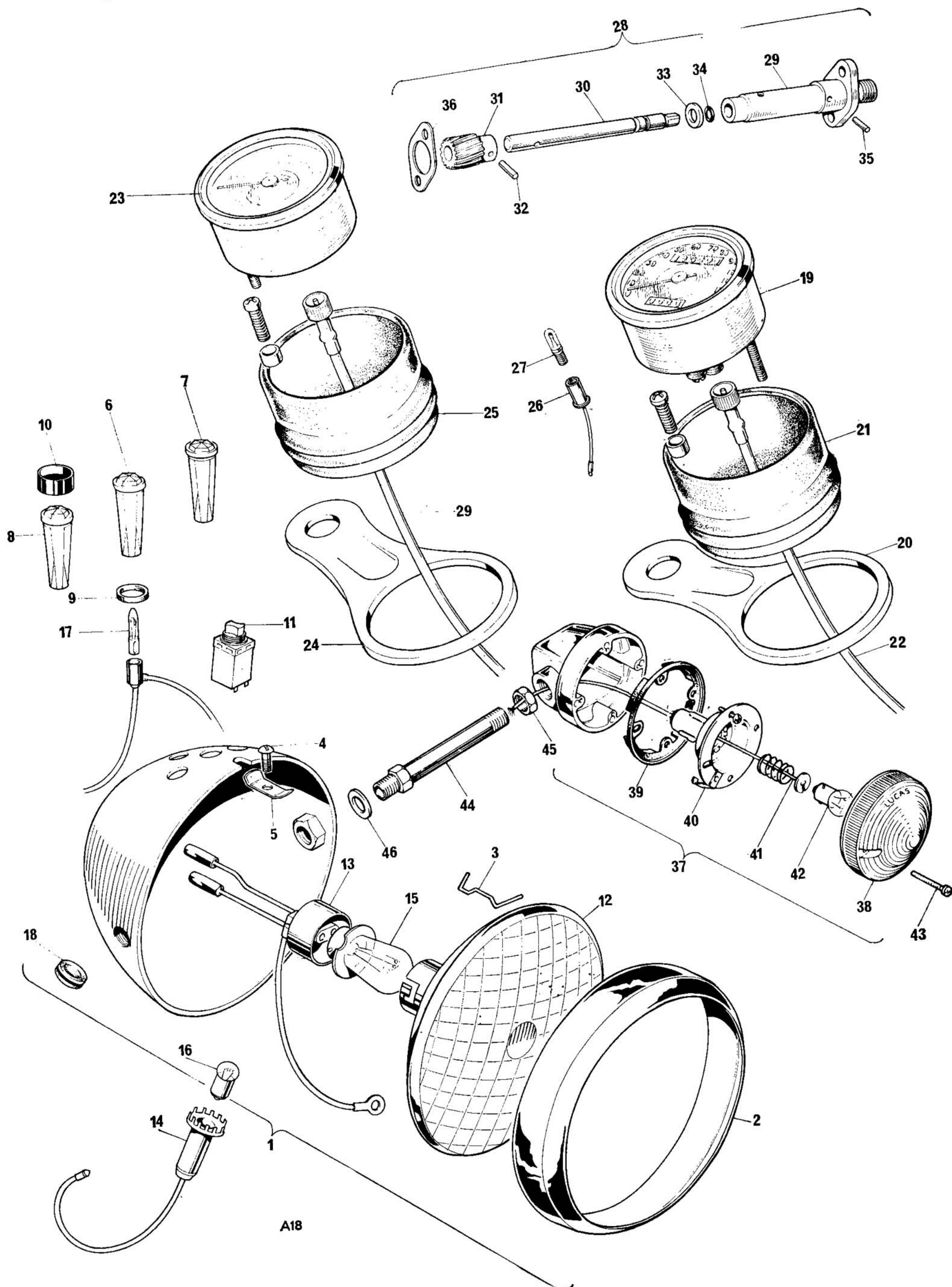
Fig. 18. HEADLAMP, SPEEDOMETER, TACHOMETER
