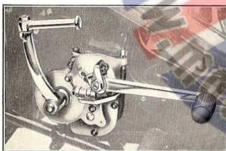
GEARBOX
