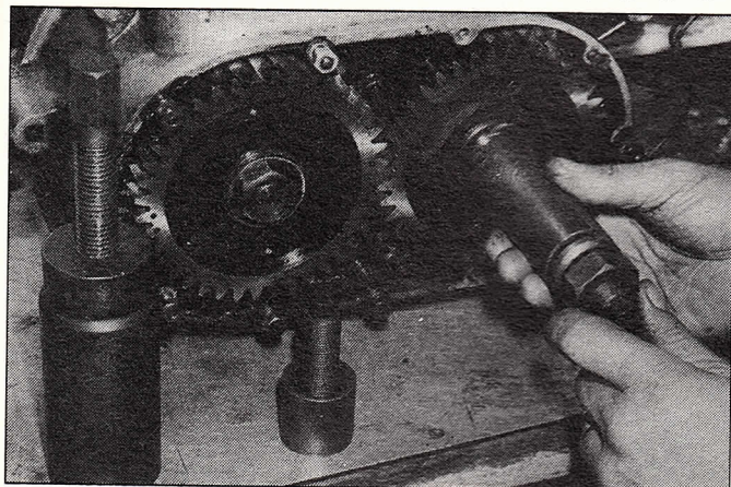
Special tools are required to remove and replace coupling gears. Front gear nut is a normal right hand thread.
