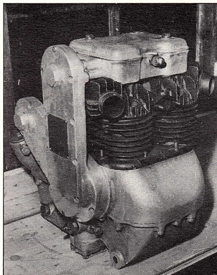
First of the line. The 1931 500cc OHC Square Four engine.
