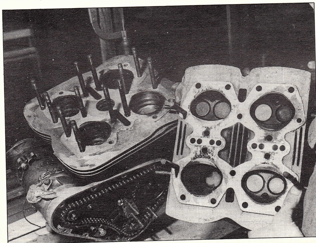
Four nuts (two each side) must be removed before removing head.
