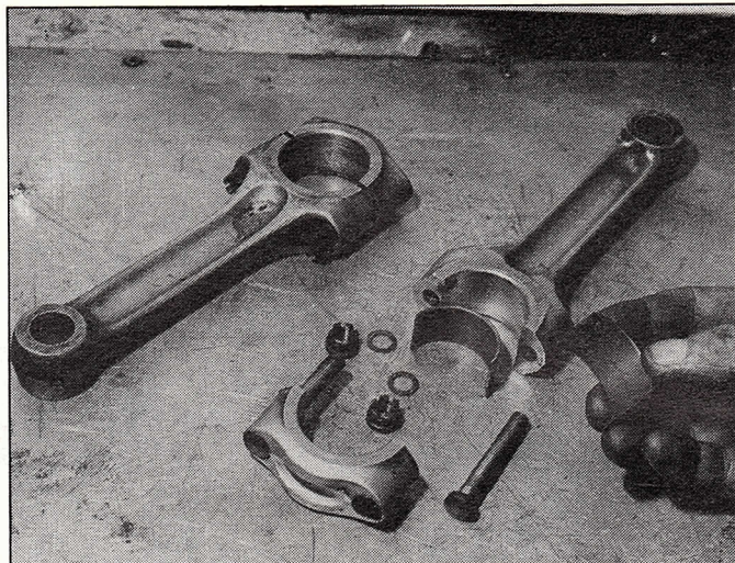
Conrods on the 1000cc Fours had detachable white metal shells, with the rods secured by slotted type nuts and split pins which were later superseded by Simmonds pinnacle lock nuts. Note late type MkII motors had the gudgeon pin running direct in the small end eye.
