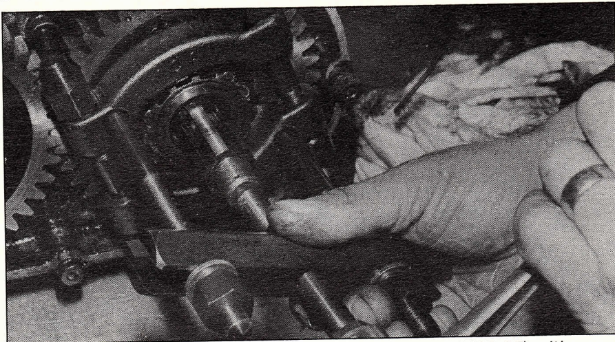
Removal of the rear crankshaft outer bearing (part no.1432-37) with 1.124in bore. Bearings in crankcase (part no.1431-37) have 1.125in bore and must not be interchanged with 1432-37.
