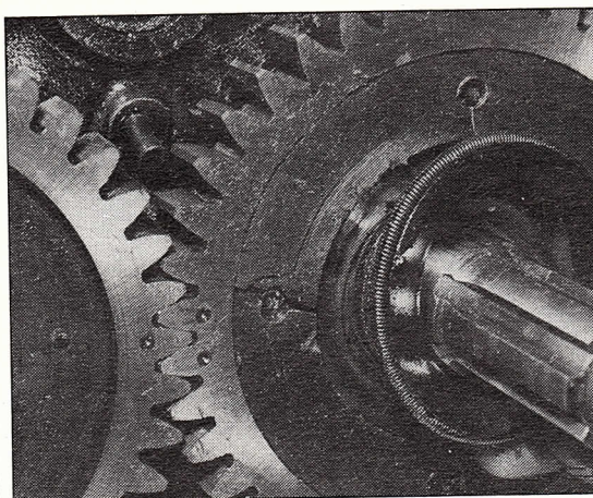
Removal of the rear crankshaft outer bearing (part no.1432-37) with 1.124in bore. Bearings in crankcase (part no.1431-37) have 1.125in bore and must not be interchanged with 1432-37.
