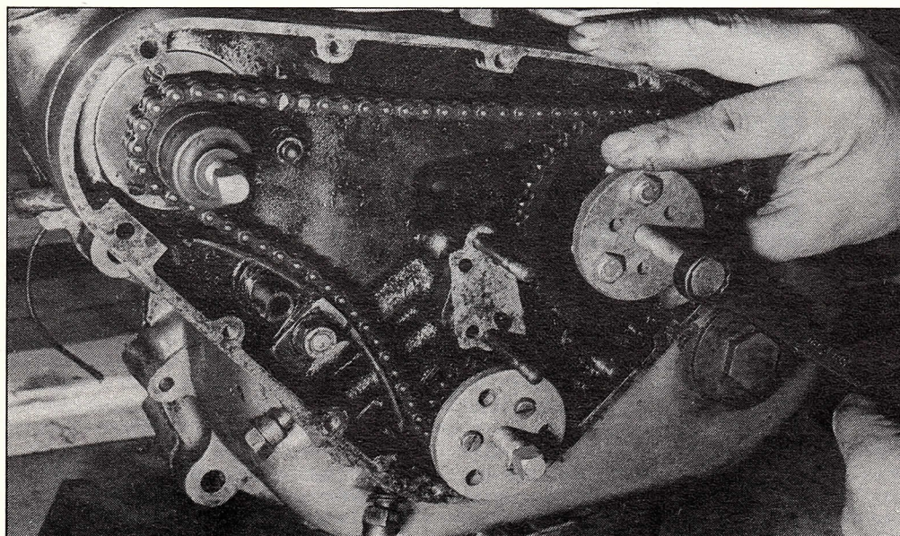
Removal of oil pump. Note steel shim between pump and crankcase joint. Note breather pipe.
