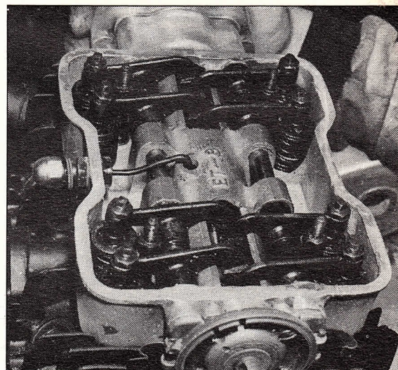
500cc OHC Four showing the overhead cam and rocker layout with distributor driven off the end of the camshaft.
