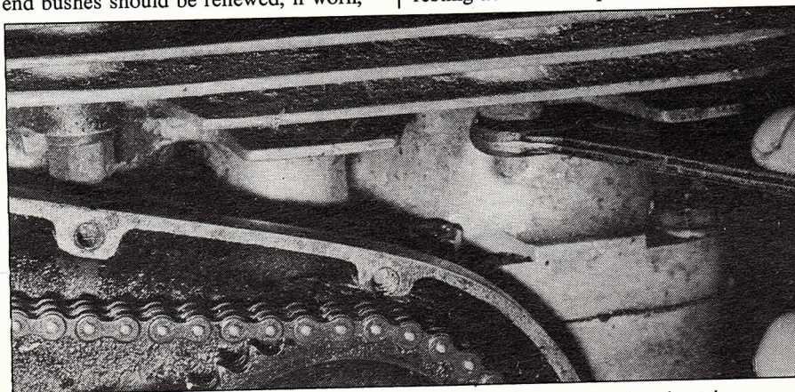
Four nuts (two each side) must be removed before removing head.
