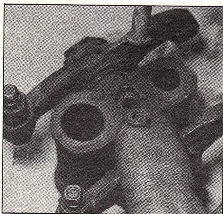
These small fibre washers must be fitted in recess in rocker pivot block to ensure oil tight joint for rocker spindle oil feed pipe.
